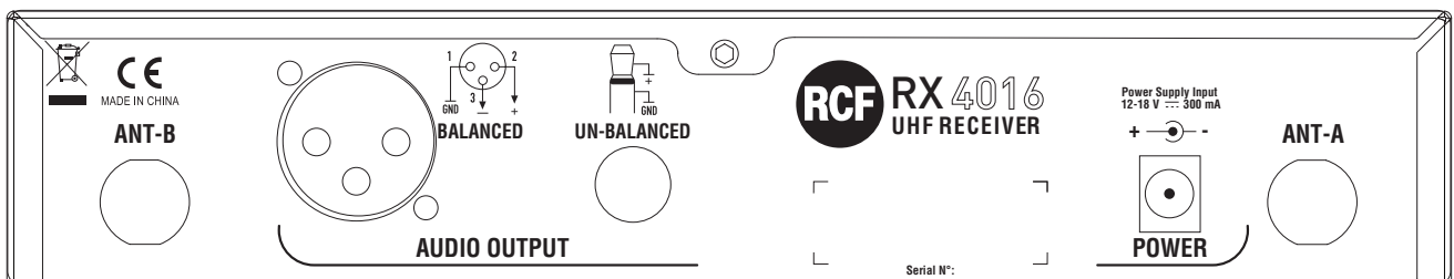
Rear panel
