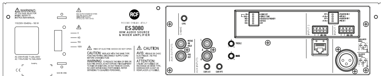
Rear panel
