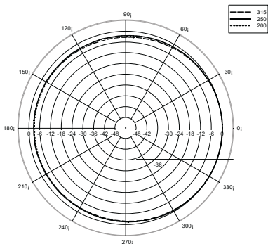
Vertical 1/3 Polar Plot
