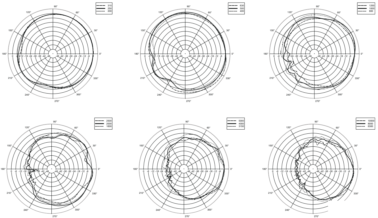
Vertical 1/3 Polar Plot
