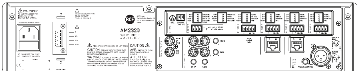
Rear panel
