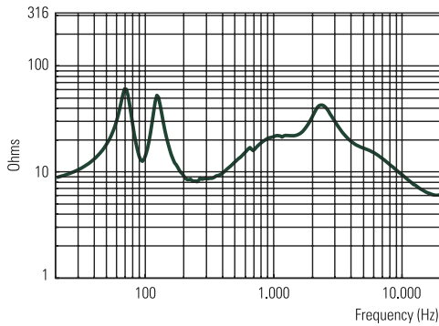
IMPEDANCE
