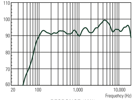
RESPONSE 1W/1m
