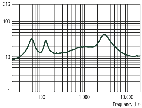
IMPEDANCE
