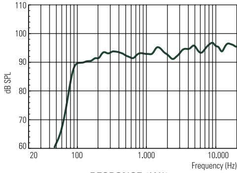
RESPONSE 1W/1m
