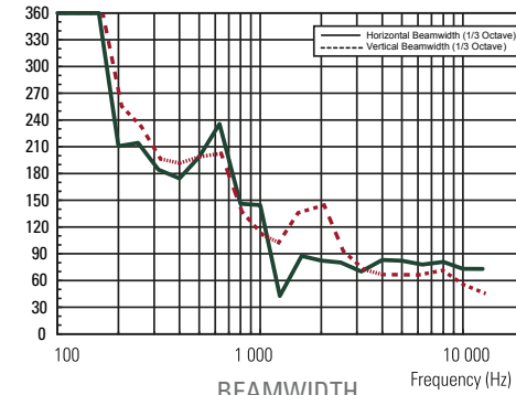
BEAMWIDTH vs. FREQUENCY
