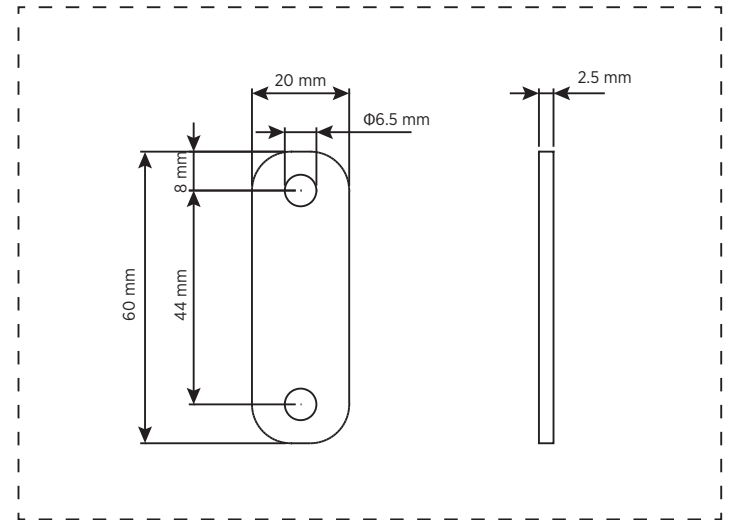
FIXING PLATE
