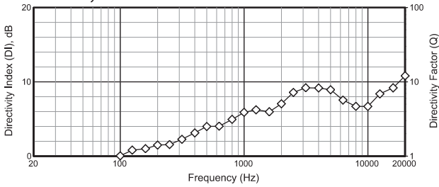
Directivity Index
