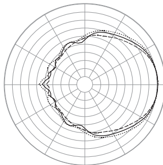
Vertical 4000 Hz 1/3 Octave Polars
