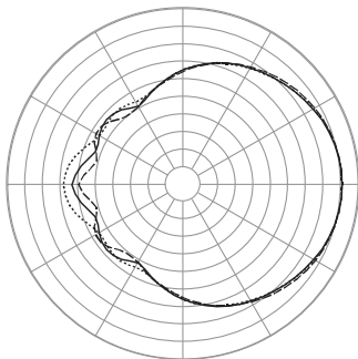
Vertical 2000 Hz 1/3 Octave Polars
