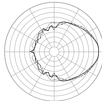
Vertical 8000 Hz 1/3 Octave Polars
