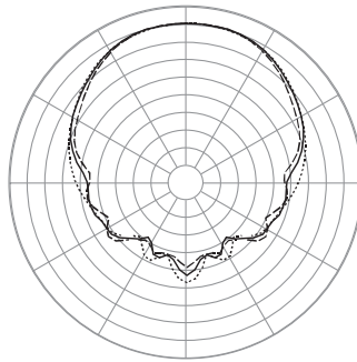
Horizontal 4000 Hz 1/3 Octave Polars
