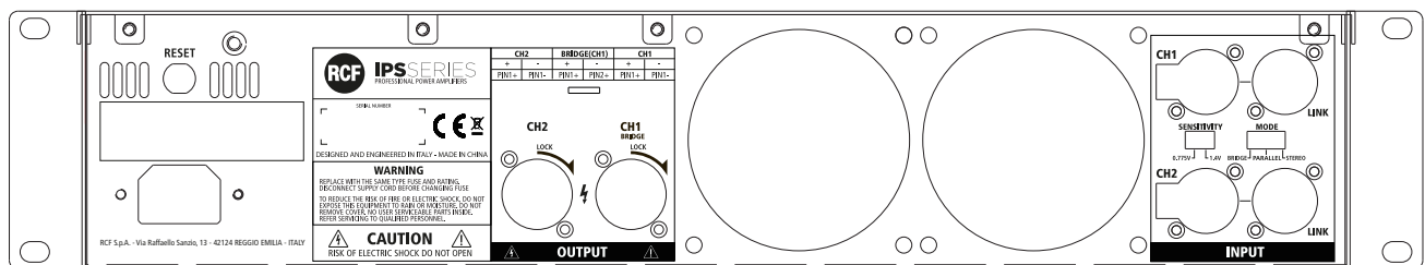
Rear panel
